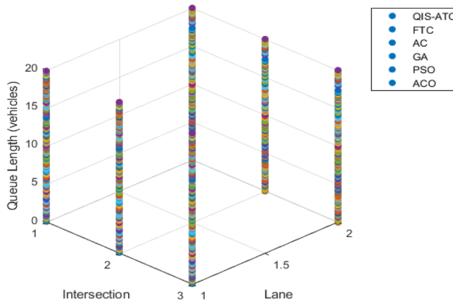
Fig 4. Plot Of Queue Length Per Lane and Intersection.
