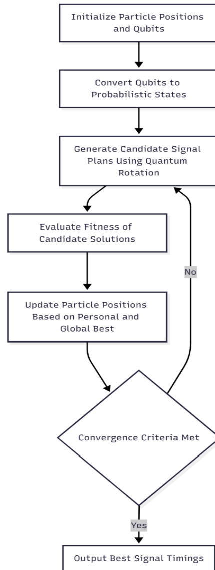
Fig 3. Quantum-Inspired Swarm Update Mechanism for Traffic Signal Optimization.
