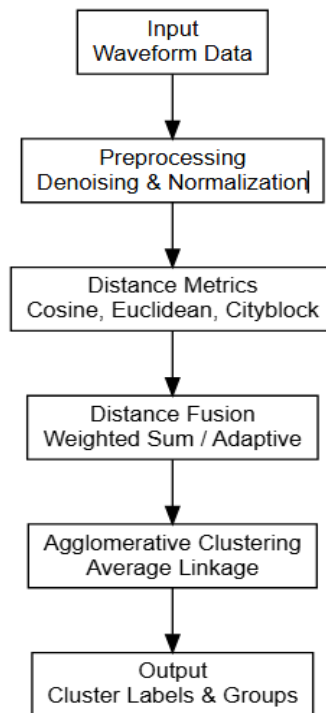
Fig 1. Block Diagram of the Proposed IMAC-Net Framework.
