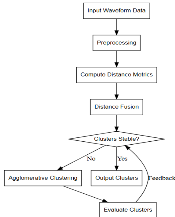
Fig 2. Flowchart of IMAC-Net Operational Workflow.
