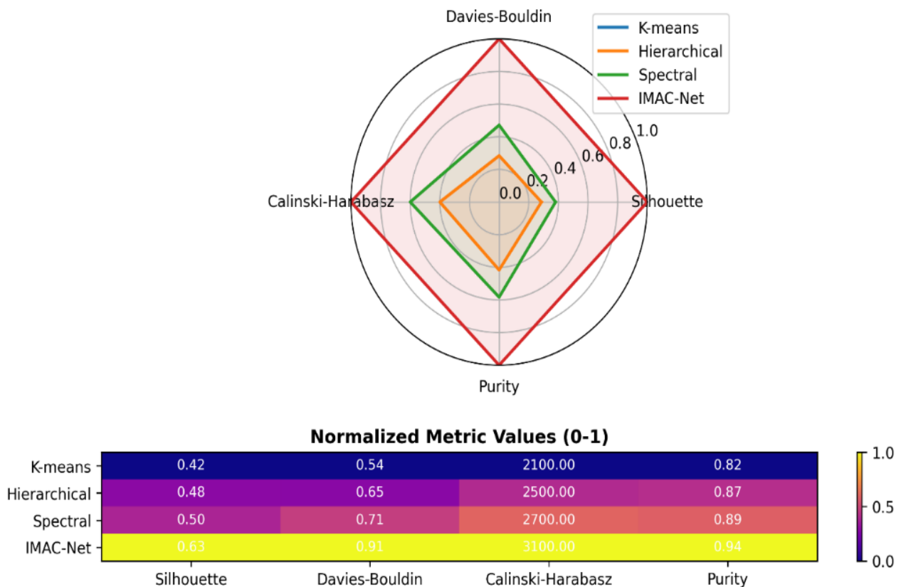
Fig 8. Comparative Performance of Clustering Methods.
