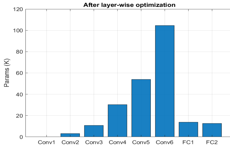
Fig 5. After Layer-Wise Optimization — Parameters Per Layer.
