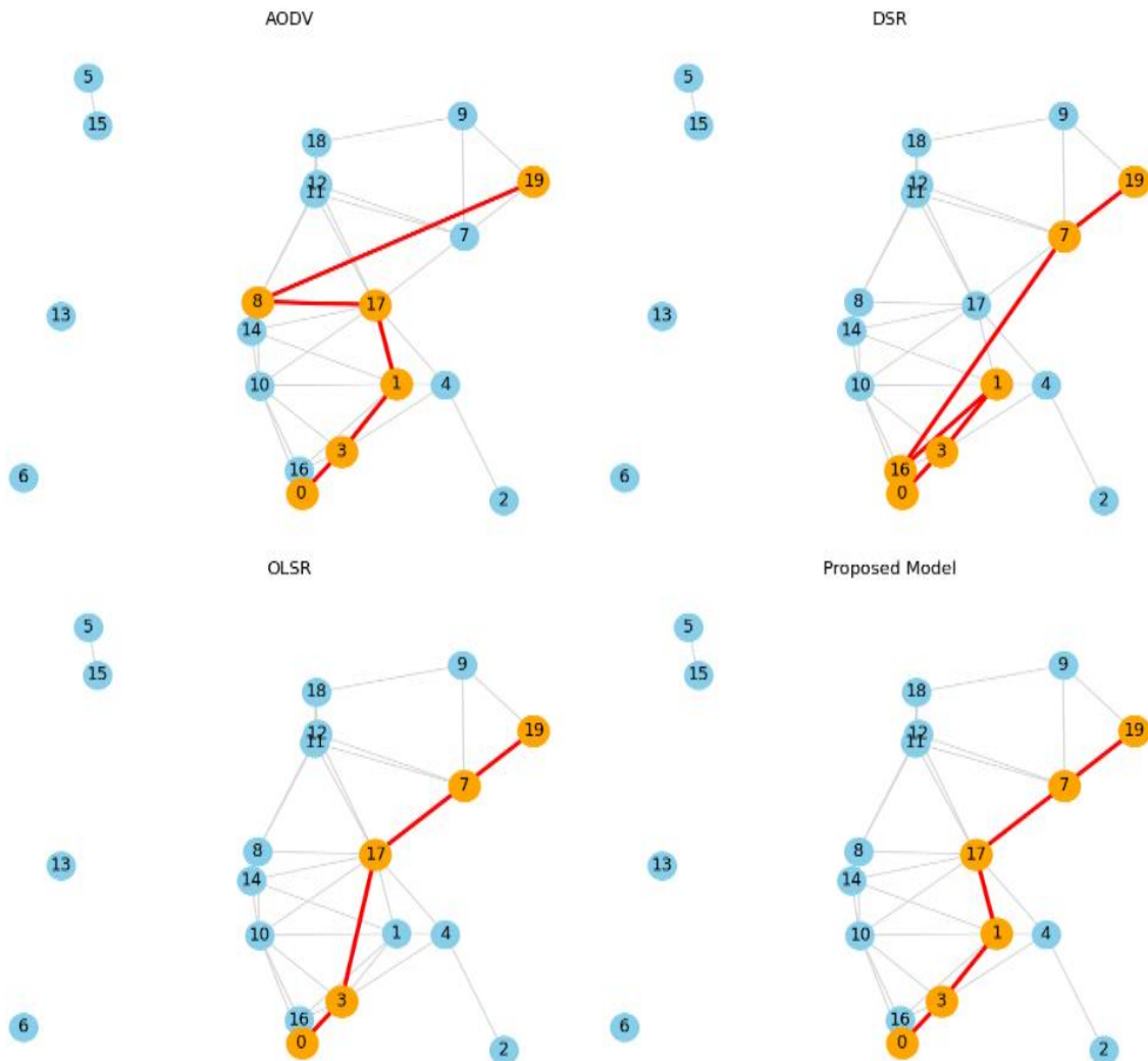
Fig 3. Routing Path Comparison (AODV, DSR, OLSR, Proposed Model).
