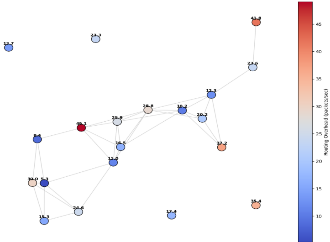
Fig 6. Routing Overhead Spread Across Nodes.
