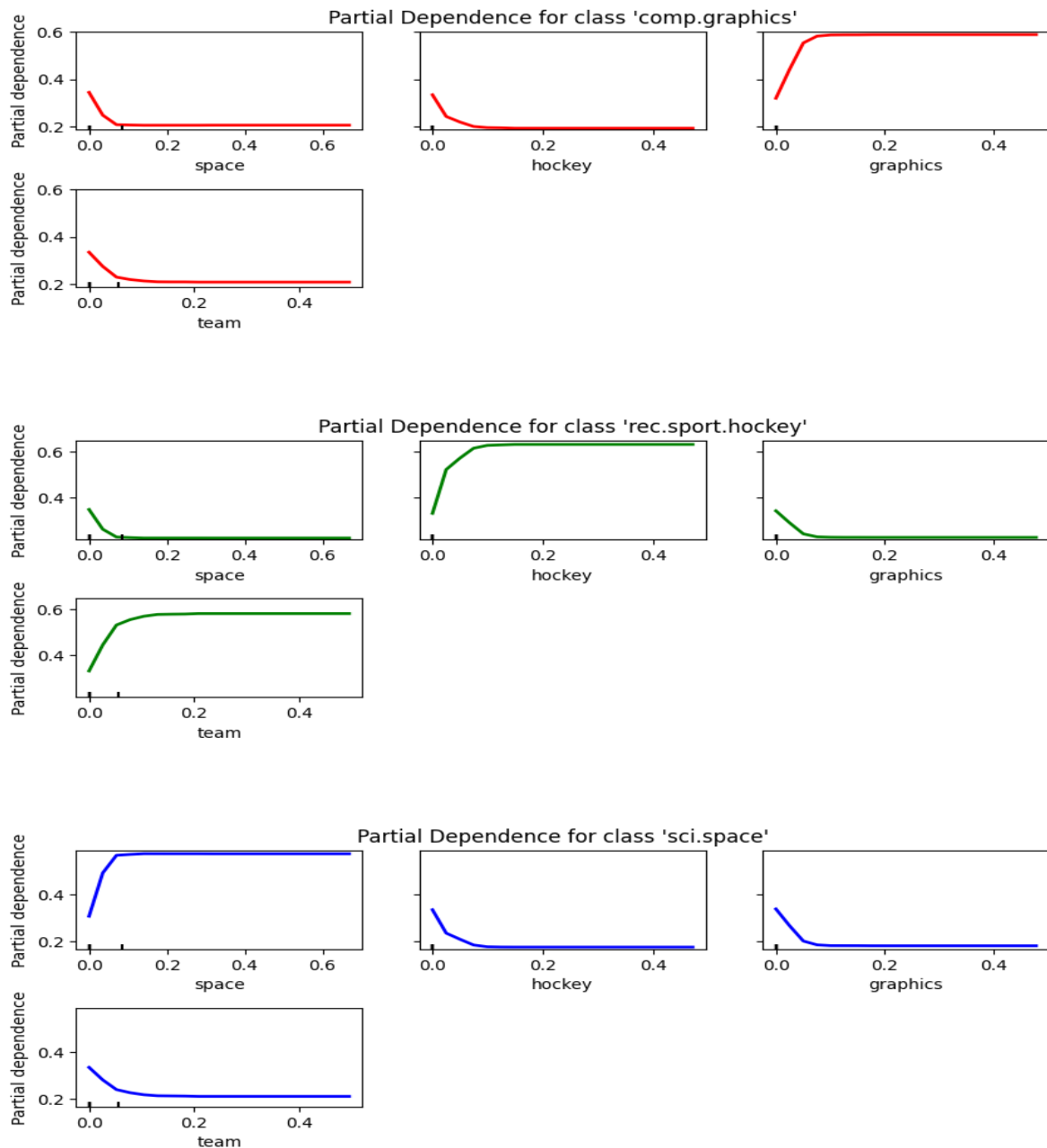
Fig 3. Partial Dependence of 20 Newsgroups Classification on Key Words.
