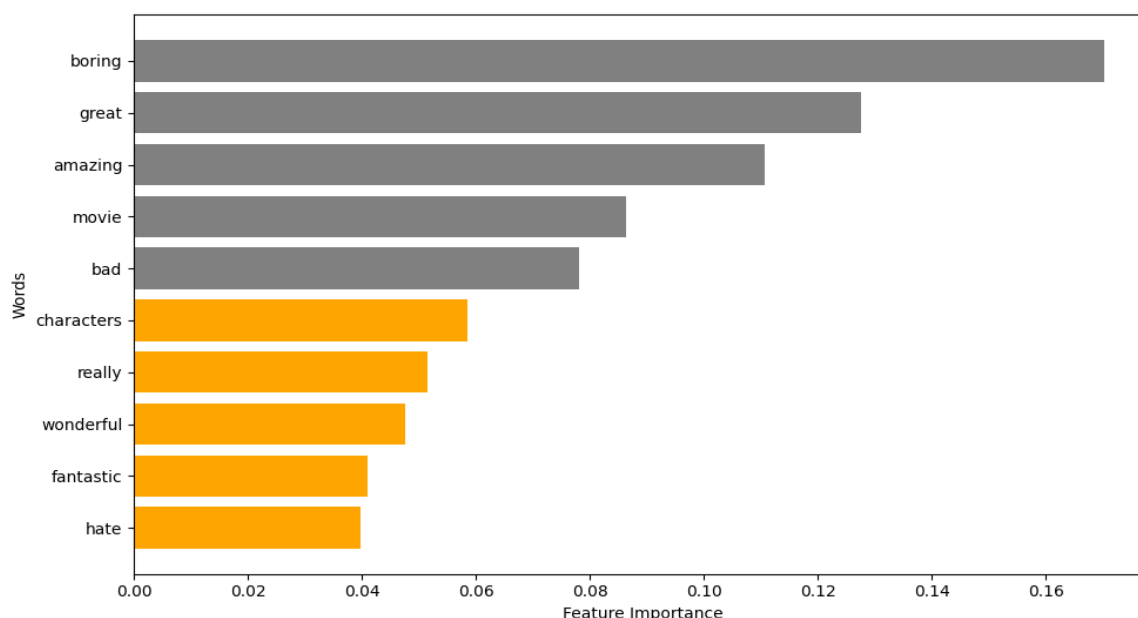
Fig 2. Top Influential Words Selected for Partial Dependence Analysis.
